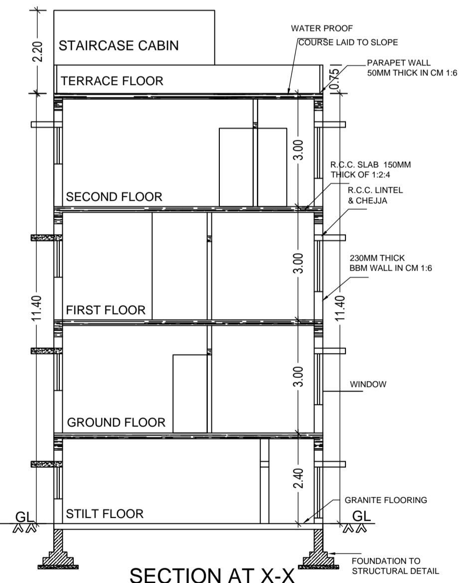
SECTION AT X-X
